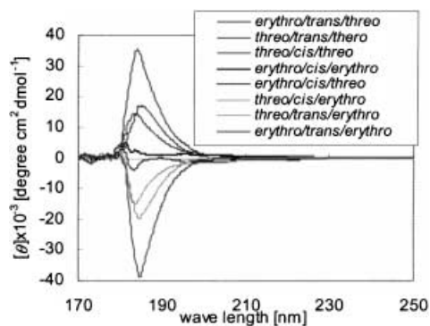
Figure 1. CD spectral data for 36–39 a and 36–39 b .
